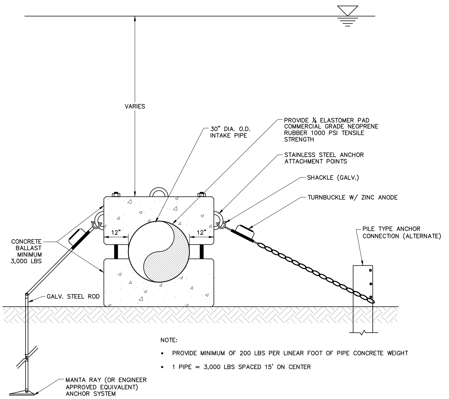
4A UNDERWATER ZONE (STATIONS 68+90 TO 69+25) NOT TO SCALE CONCEPTUAL NOT FOR CONSTRUCTION
