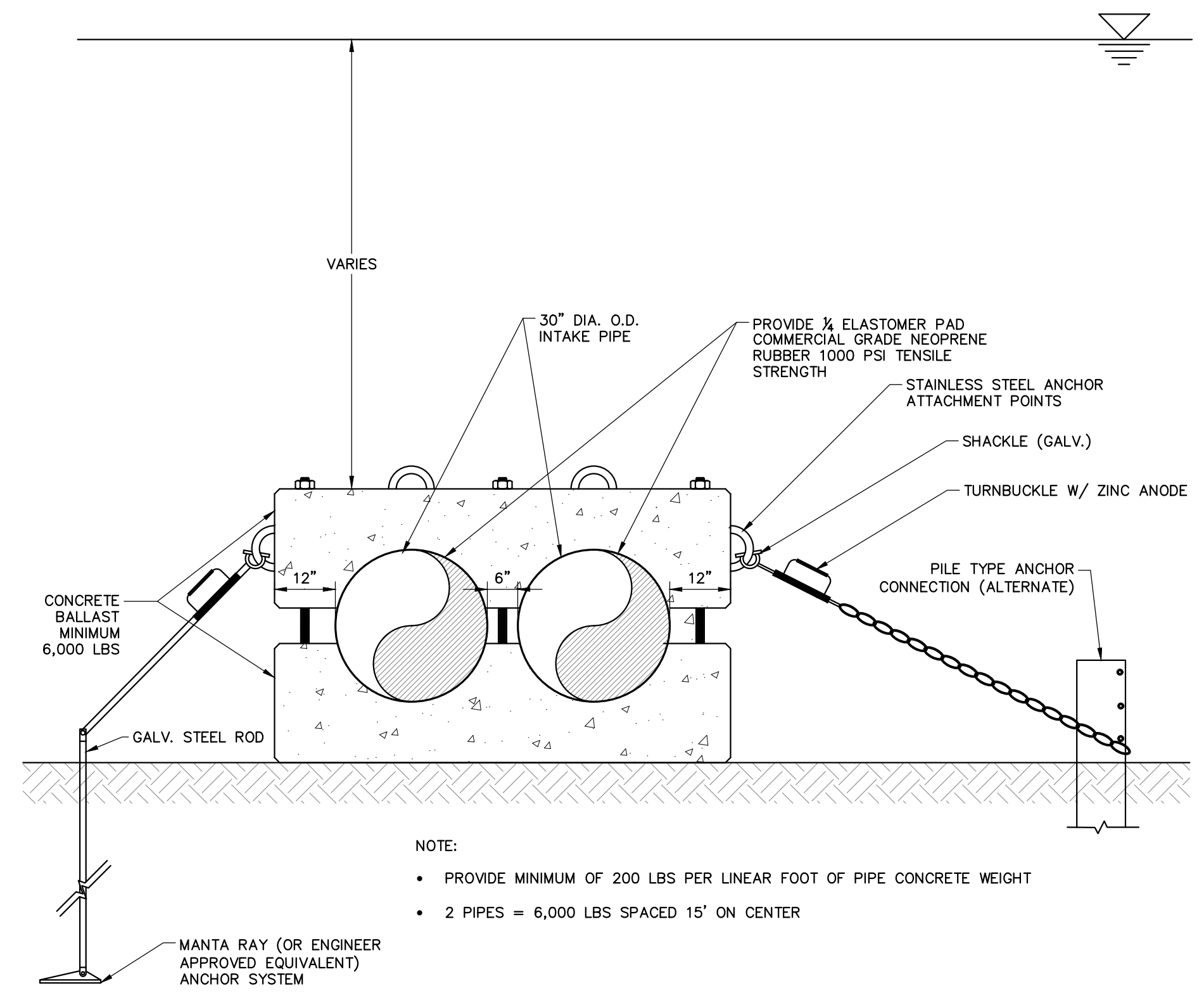
4 UNDERWATER ZONE (STATIONS 42+00 TO 68+90) NOT TO SCALE CONCEPTUAL NOT FOR CONSTRUCTION
