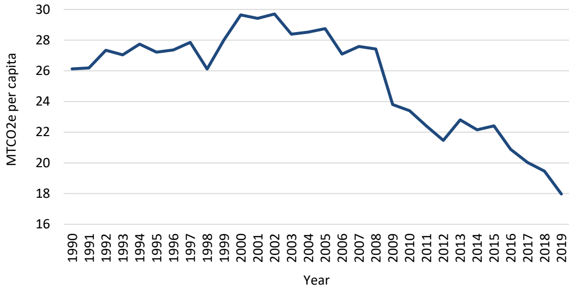
Figure A2. Maine's greenhouse gas emissions per capita 1990-2019 (GHG emissions include biogenic emissions)
